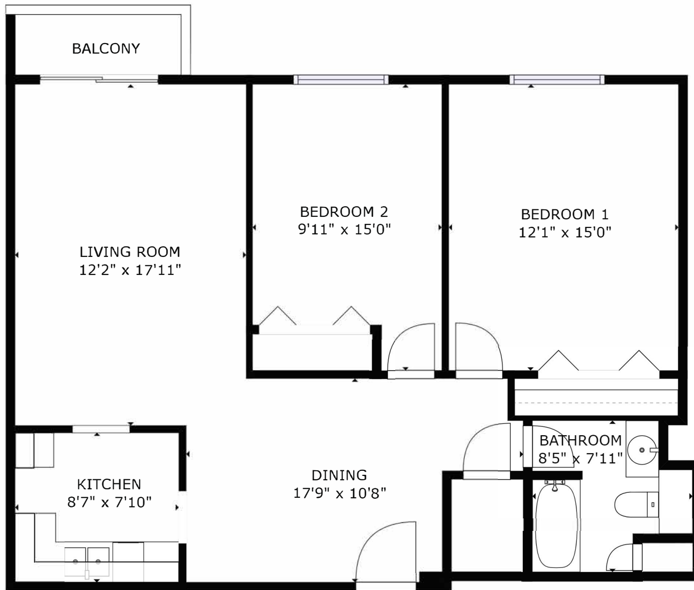
FLOOR 1
